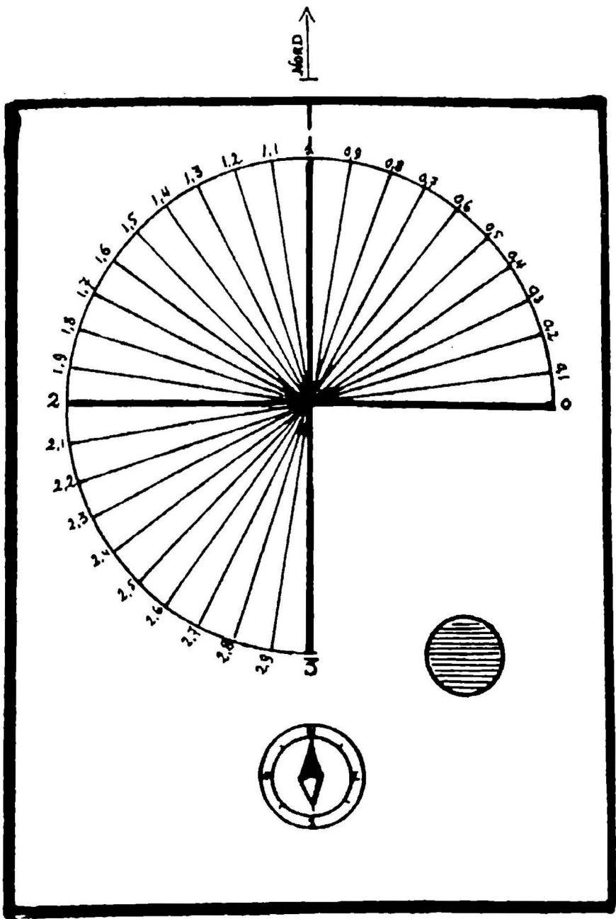
Figure 20: The Micrometer, north to the top
